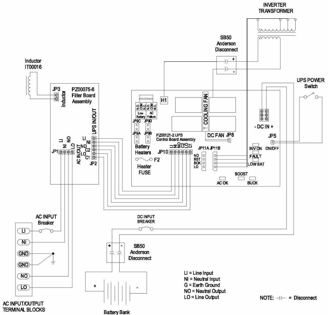
Figure 4: Outdoor XUPS-600A/B-1000A/B Wiring Diagram
