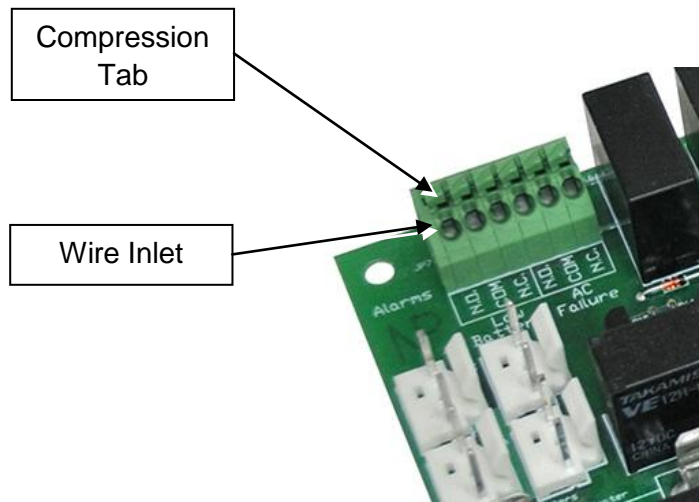
Figure 9: Alarm Connections
