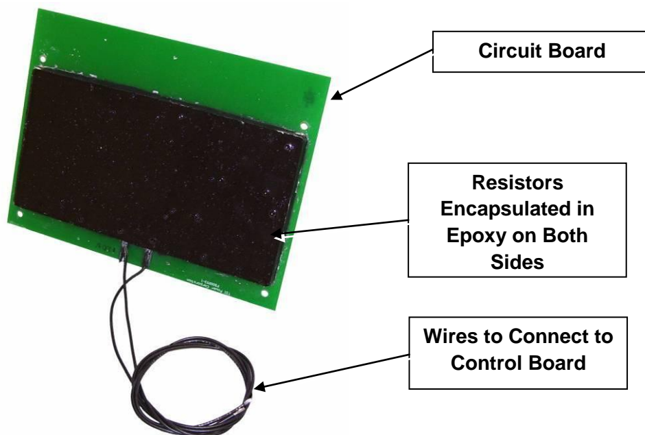
Figure 18: Optional Battery Heater Circuit Board
