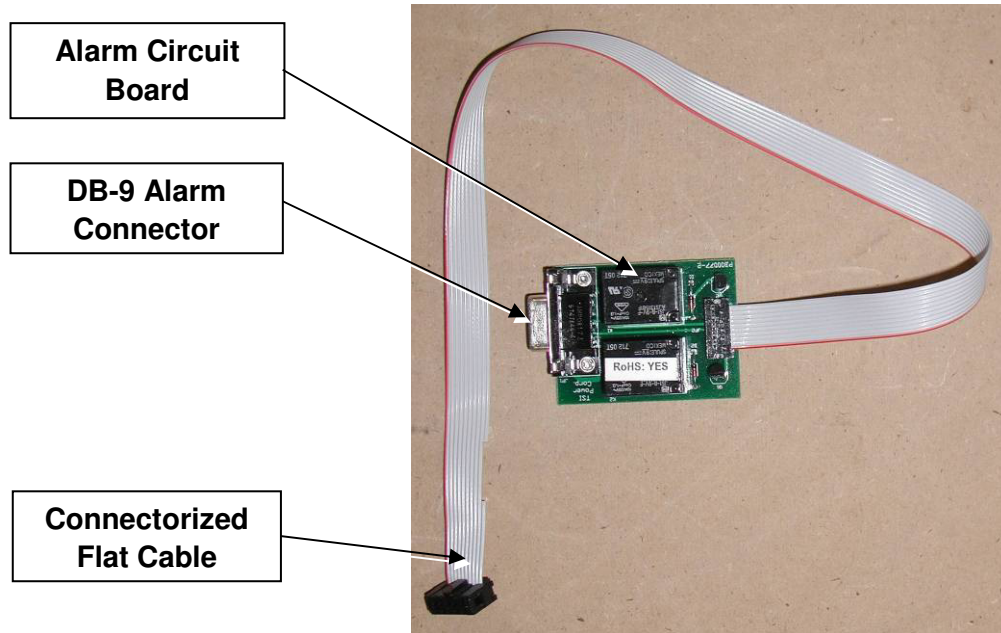
Figure 10: Alarm Circuit Board
