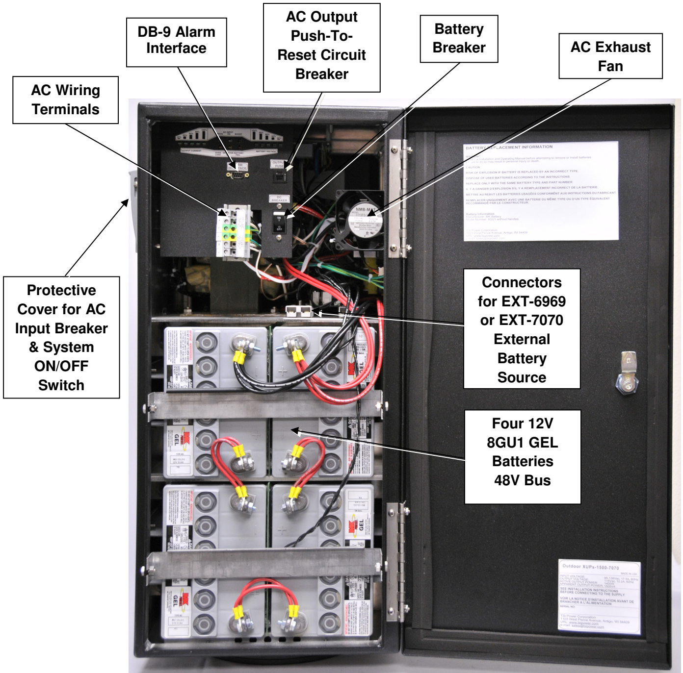
Figure 3: Electronic Compartment
