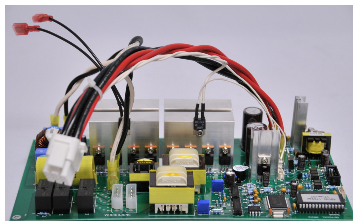
Figure 7: Main Inverter, Charging & Voltage Regulation Circuit Board
