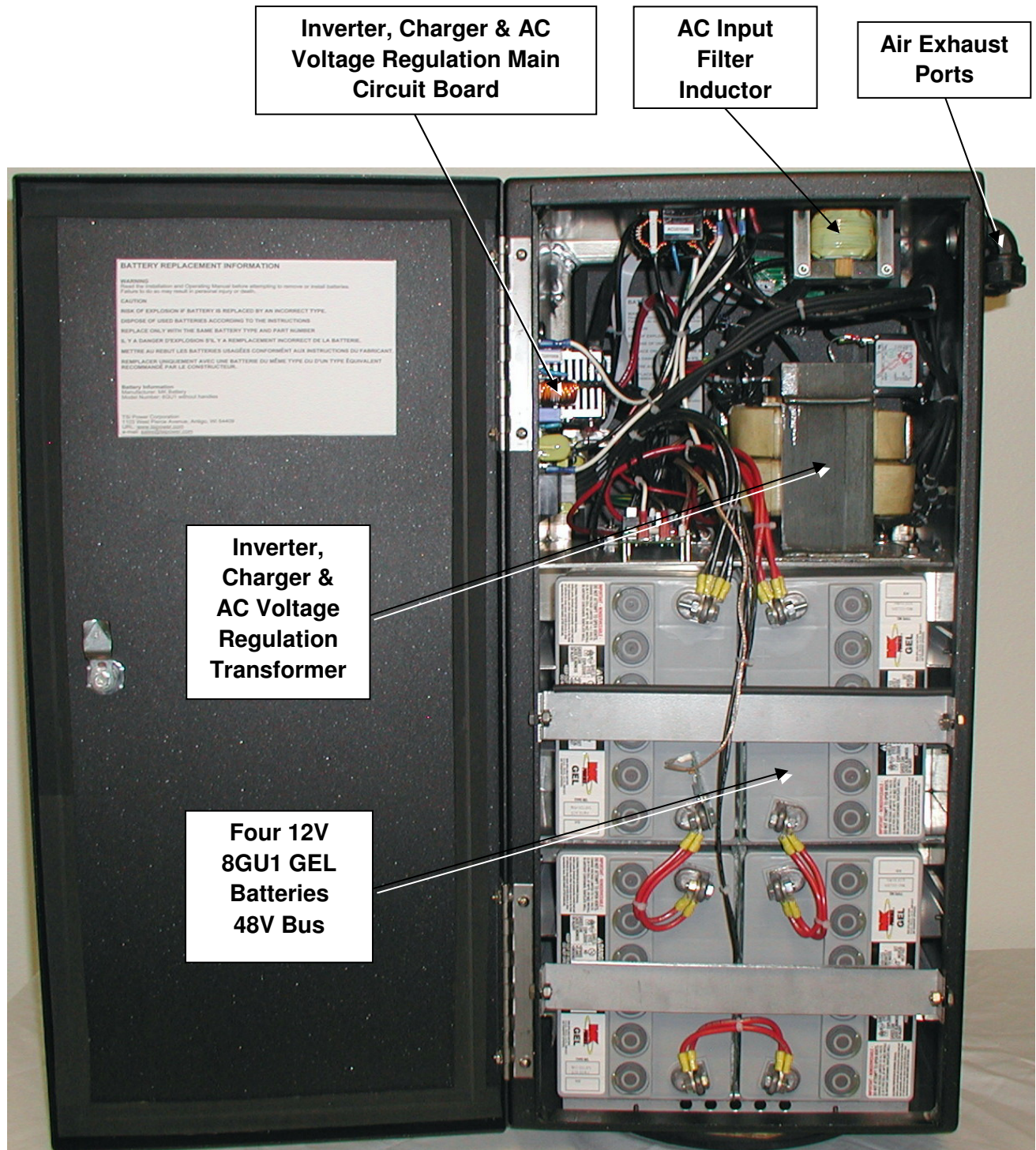
Figure 4: Electronic and Battery Compartment
