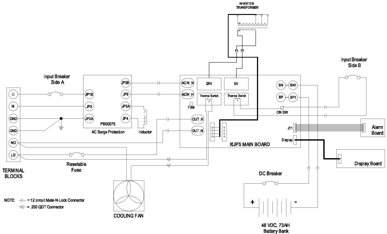
Figure 5: XUPS-1500-7070 Wiring Diagram
