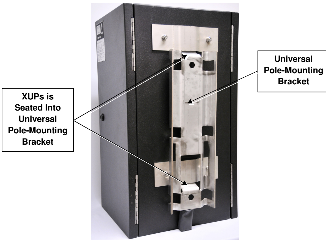
Figure 14: Universal Pole-Mounting Bracket
