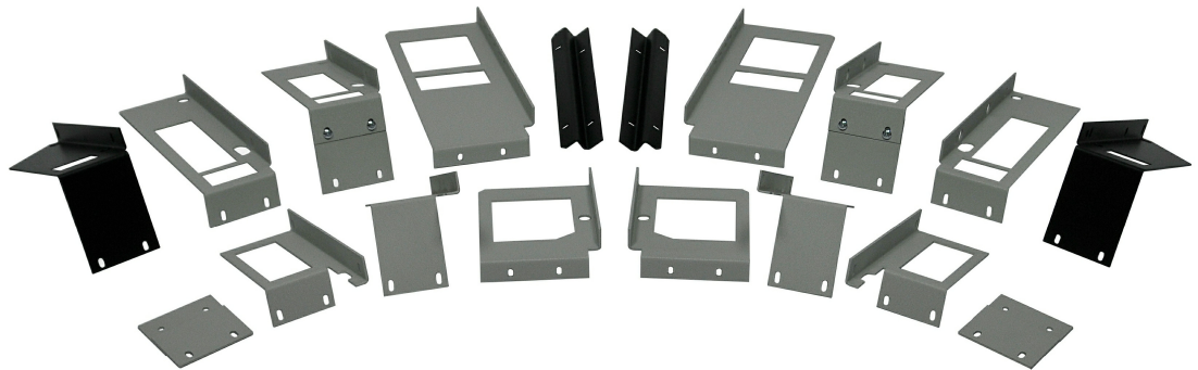
Front, center and rear rack-mounting brackets for 19", 23" and 24" racks, as well as wall and floor mounting brackets
